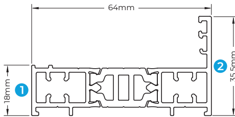
SC100 SMALL OUTER FRAME
