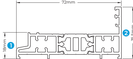
SC101 FLUSH SMALL OUTER FRAME
