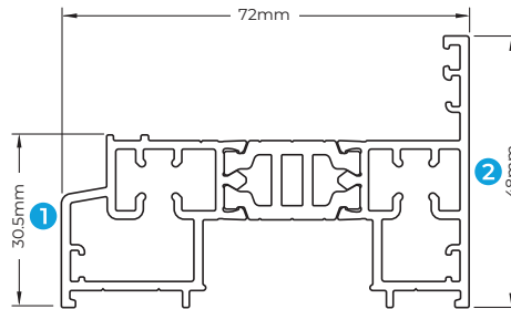
SC103 FLUSH INTERMEDIATE OUTER FRAME
