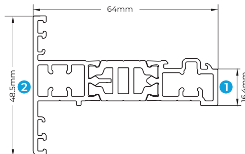
SC311 CONTEMPORARY BEADED SASH
