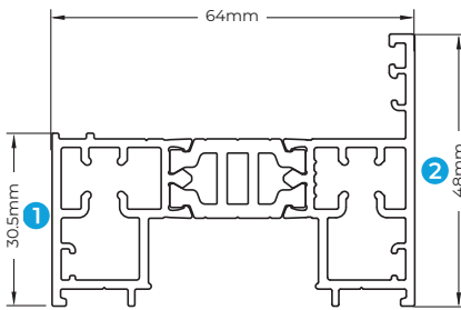
SC102 INTERMEDIATE OUTER FRAME
