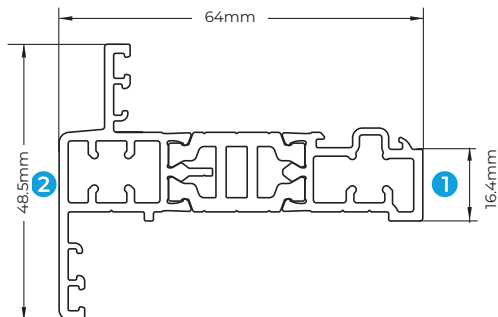
SC310 STEPPED BEADED SASH
