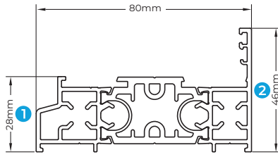
SP101 SMALL FLUSH OUTER FRAME
