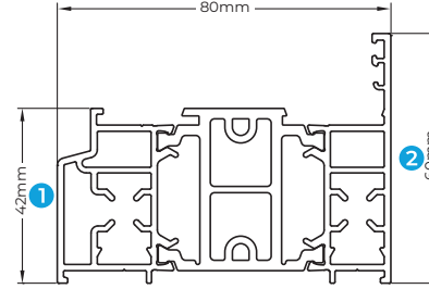
SP103 INTERMEDIATE FLUSH OUTER FRAME
