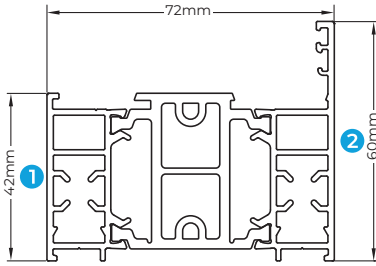
SP102 INTERMEDIATE OUTER FRAME
