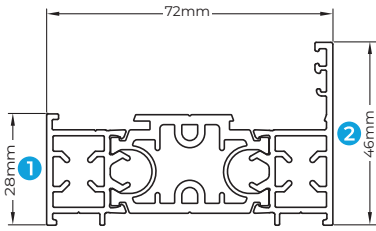
SP100 SMALL OUTER FRAME
