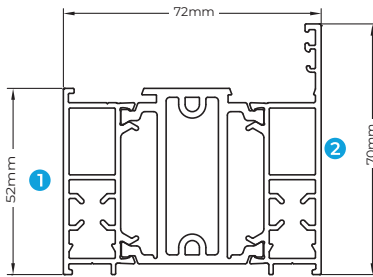
SP104 LARGE OUTER FRAME
