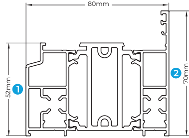
SP105 LARGE FLUSH OUTER FRAME
