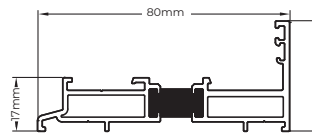
SP702 FRAME LOW THRESHOLD Tested to the requirements of Part M
