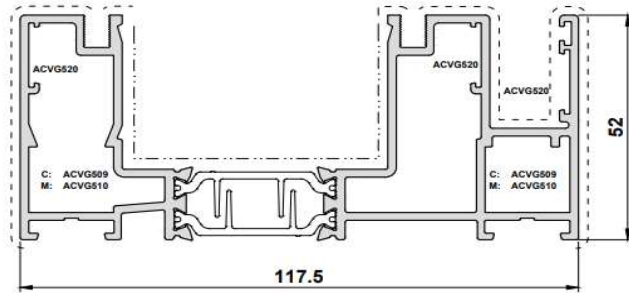
VG511N Two Track Outer Frame with Upstand
